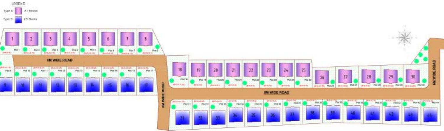
MASTER PLAN Total Site Area = 86834.23 Sq. Ft.
